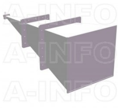
LB-137-25-C-7SPO Standard Gain Horn Antenna 5.85-8.2GHz 25dB Gain 7mm
