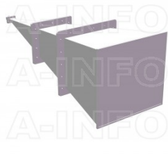
LB-137-25-C-3.5FSPO Standard Gain Horn Antenna 5.85-8.2GHz 25dB Gain 3.5mm Female
